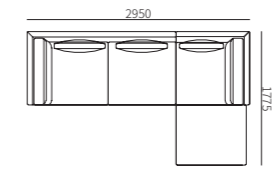
尺寸: 2950*1775*740mm
